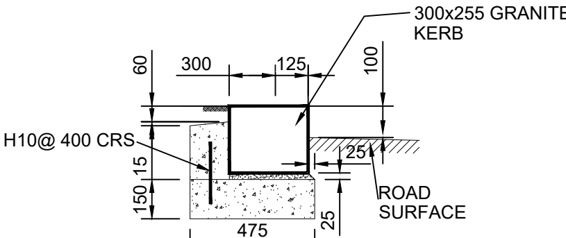
KERB TYPE K1 SCALE 1:20
